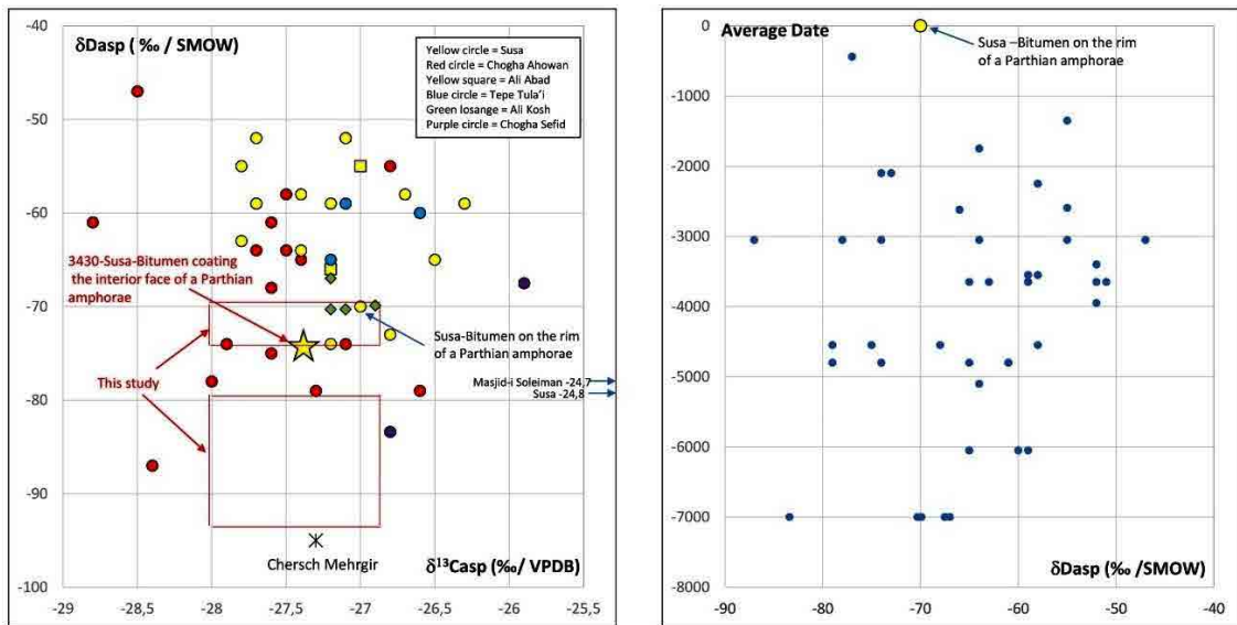
Fig. 29: Plot of \delta D_{asp} (‰ / SMOW) vs. \delta^{13}C_{asp} (‰ / VPDB) of bitumens from archaeological sites used as proxis. Plot of \delta D_{asp} (‰ / SMOW) as a function of date of samples from archaeological sites.
